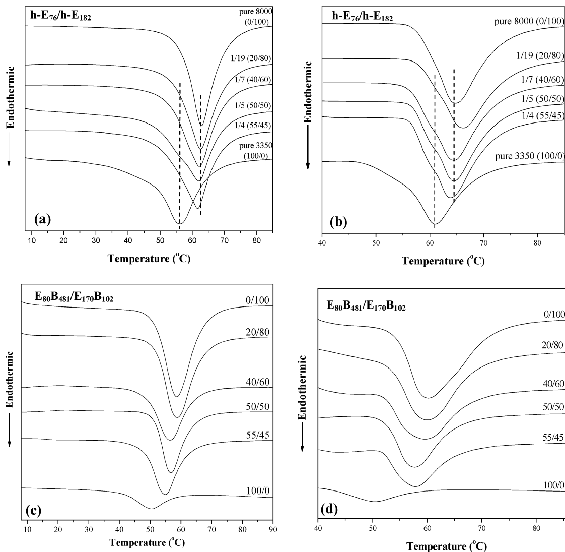
Figure 3. DSC melting curves of h-E 76 /h-E 182 and E 80 B 481 /E 170 B 102 blends obtained after isothermal crystallization at a heating rate of 20 °C/min: (a) h-E 76 /h-E 182 , T c = 8 °C; (b) h-E 76 /h-E 182 , T c = 40 °C; (c) E 80 B 481 /E 170 B 102 , T c = 8 °C; (d) E 80 B 481 /E 170 B 102 , T c = 40 °C. Each bracket in (a) and (b) indicates the corresponding composition of the diblock blend with the same mixing ratio of the shorter and the longer PEO chains as that in the homopolymer blend. The melting curves of neat E 80 B 481 in (c) and (d) were obtained after cooling the sample to −50 °C.
